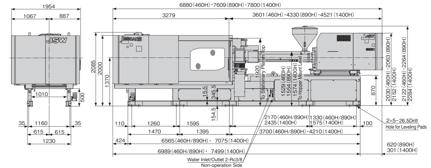
Equipment Dimensions and Mold Related Dimensions
